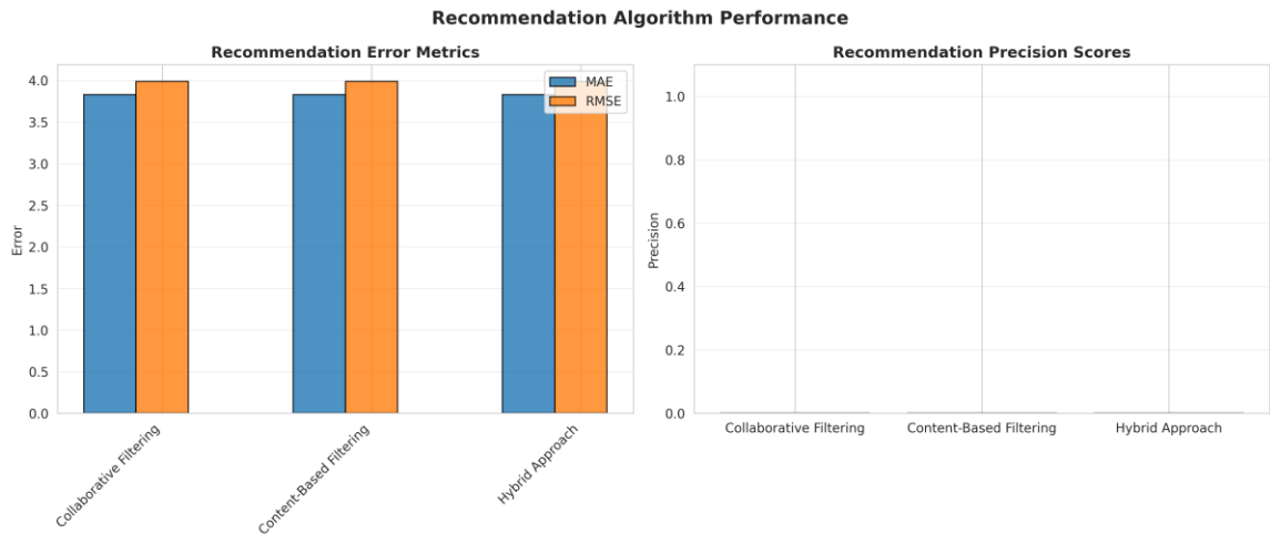
Figure 4: Recommendation Algorithm Performance Comparison
